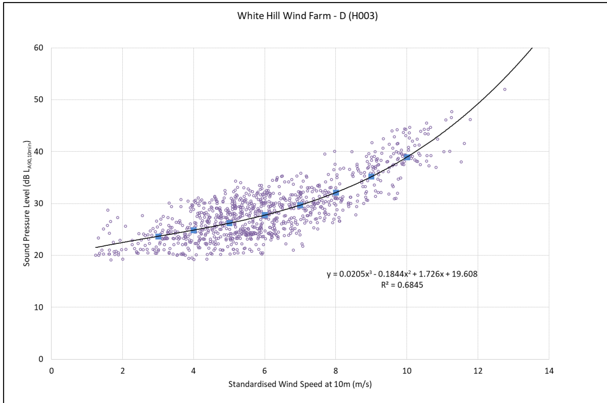
Figure 11.14: Background Noise Levels LA90,10 min dB – Location D (H003) – Daytime
