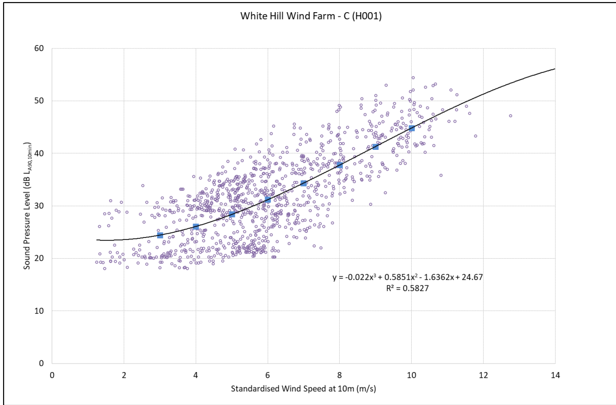
Figure 11.12: Background Noise Levels L_{A90,10 min} dB – Location C (H001) – Daytime
