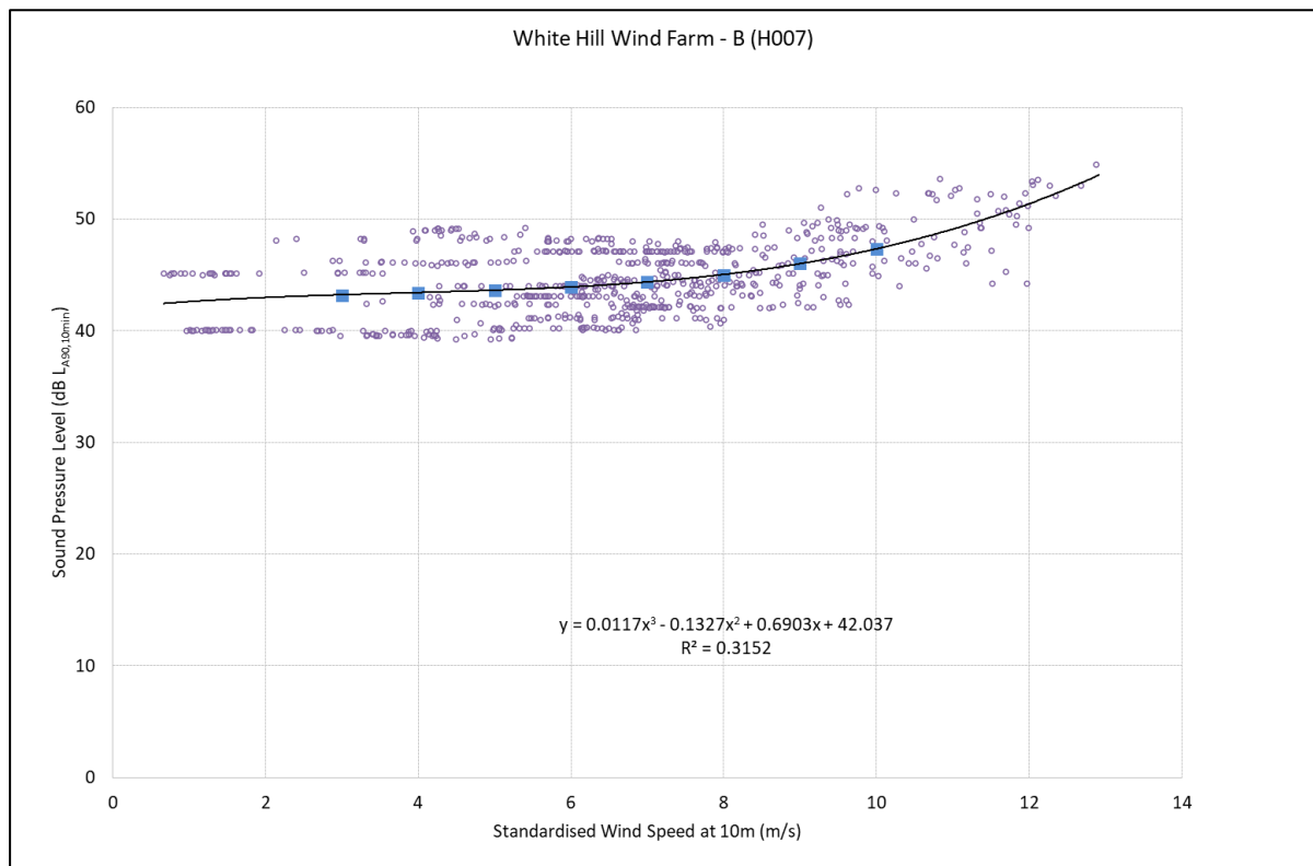
Figure 11.11: Background Noise Levels L_{A90,10 \text{ min}} dB – Location B (H007) – Night-time
