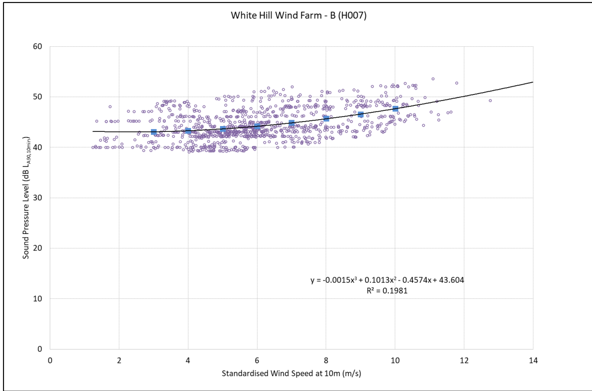
Figure 11.10: Background Noise Levels L_{A90,10 \text{ min}} dB – Location B (H007) – Daytime
