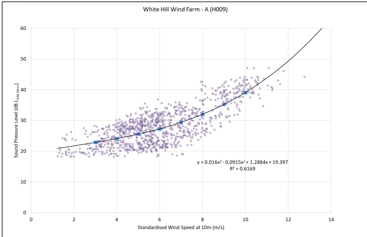
Figure 11.8: Background Noise Levels LA90,10 min dB – Location A (H009) – Daytime
