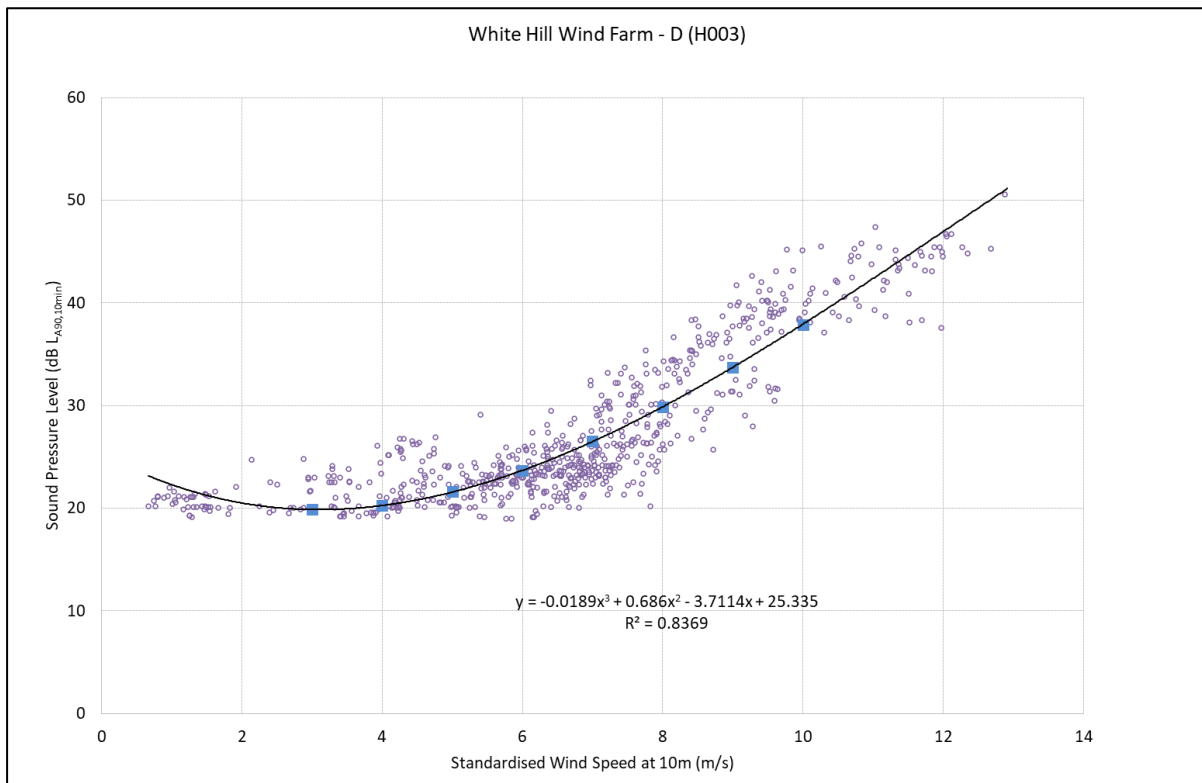
Figure 11.15: Background Noise Levels LA90,10 min dB – Location D (H003) – Night-time
