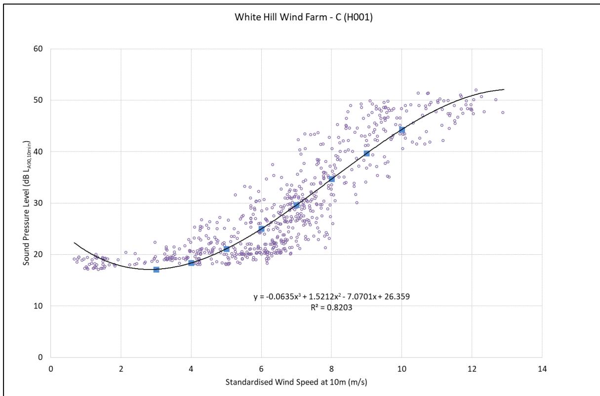
Figure 11.13: Background Noise Levels L_{A90,10 min} dB – Location C (H001) – Night-time
