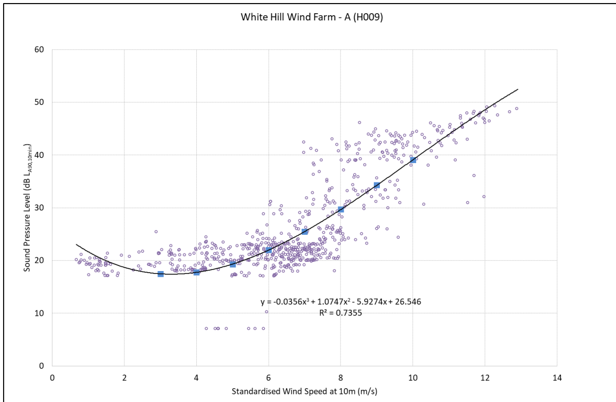
Figure 11.9: Background Noise Levels LA90,10 min dB – Location A (H009) – Night-time
